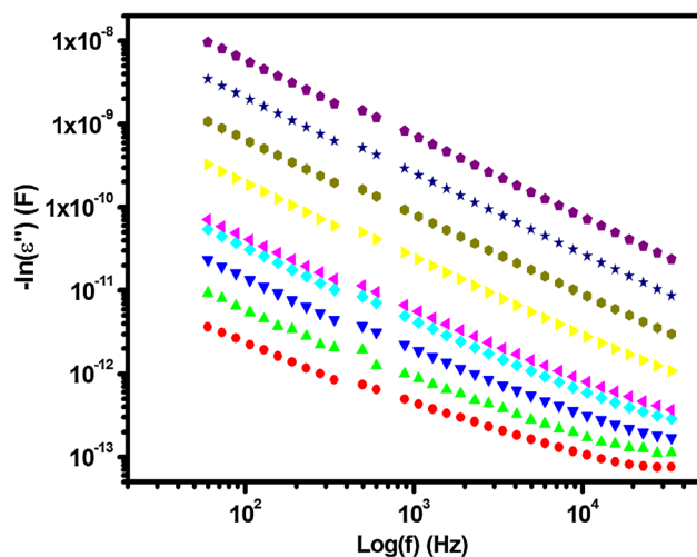
Fig. 5 The natural log of the dielectric loss as a function of frequency for all temperatures studied in this work. The figure shows the linear behavior of the dielectric loss up to f=3 \times 10^4 Hz. The non-linear behavior after this frequency is presented in the supplementary information provided online in Fig. S2
